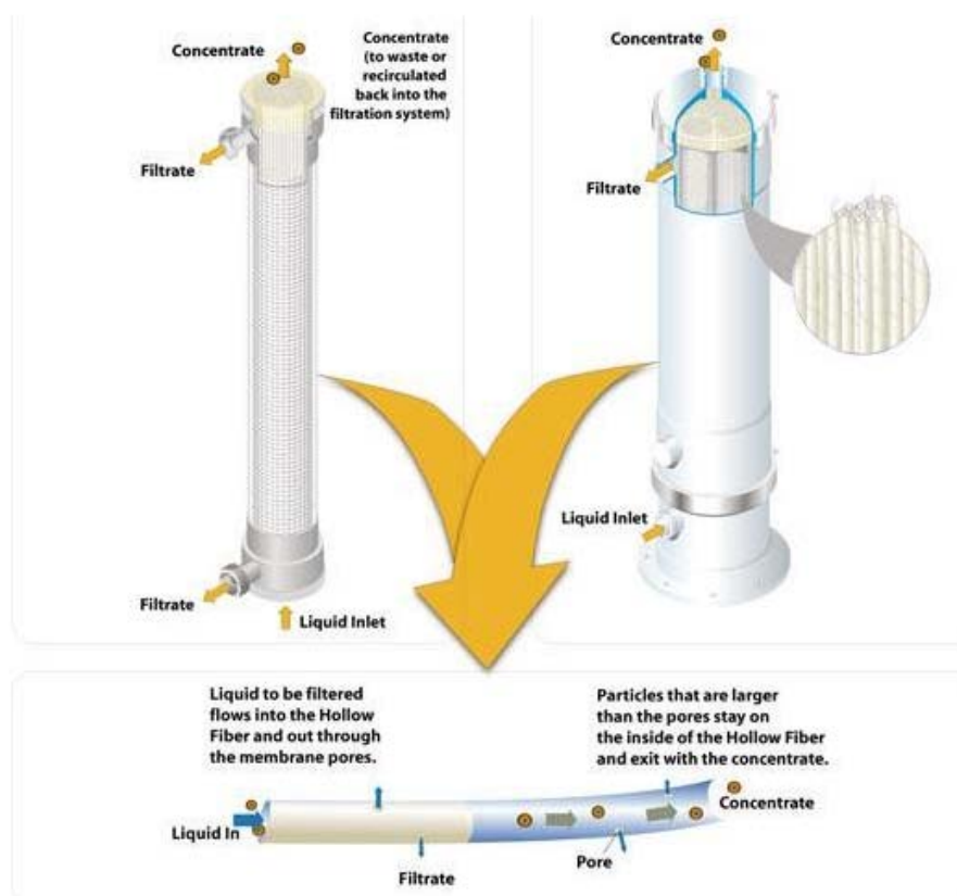
Figure 55 The Planktontrap (Photo modified from www.ballast-water.co.uk ).
