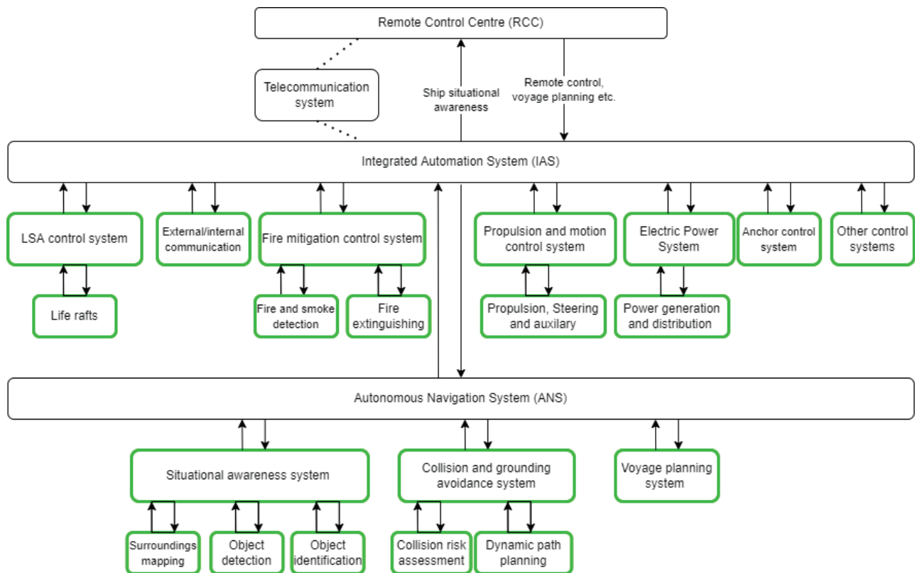
Figure 18: Small Passenger Ferry hierarchical control structure
