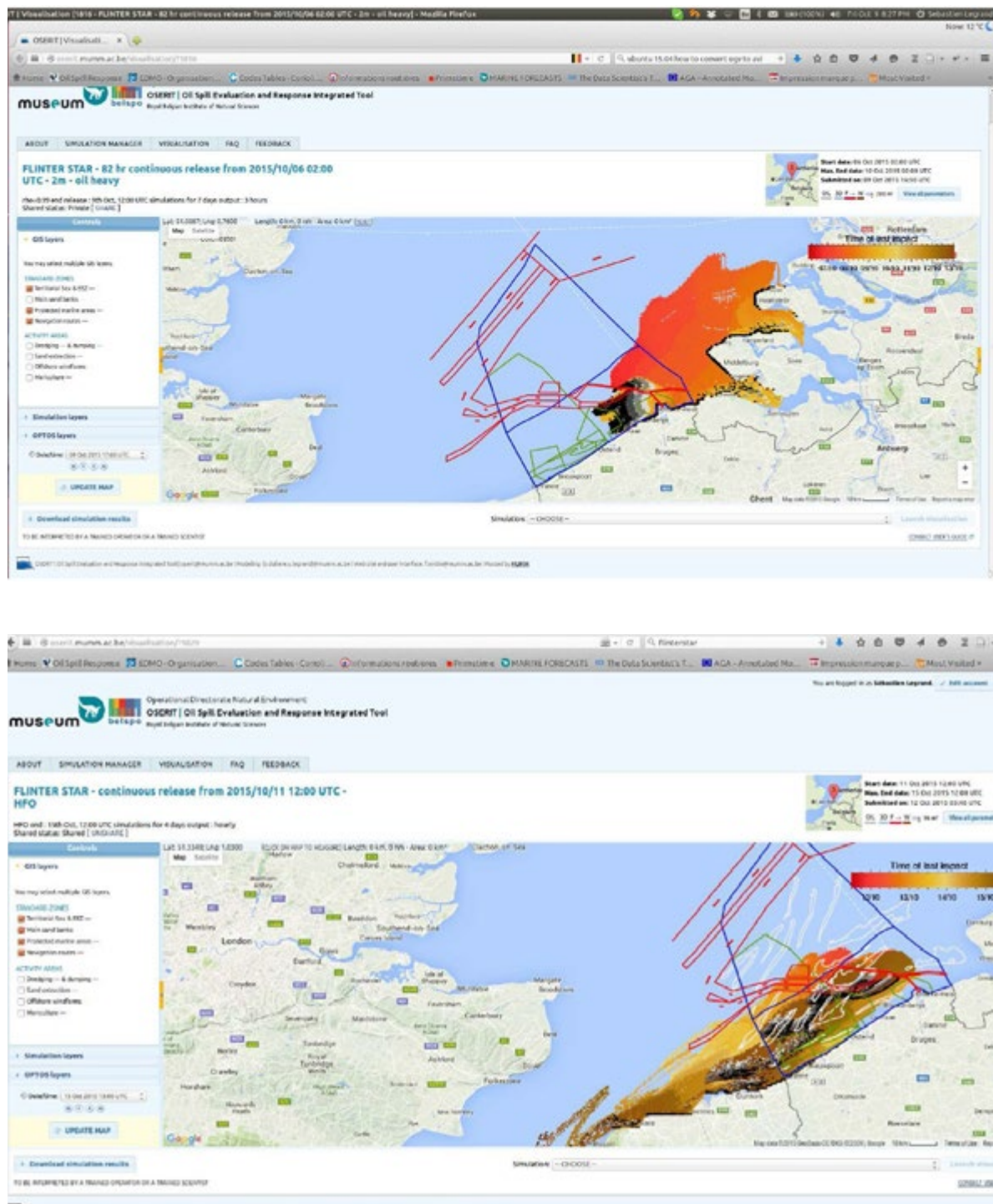
Figure 40: Oil drift simulations (worst case scenario)
