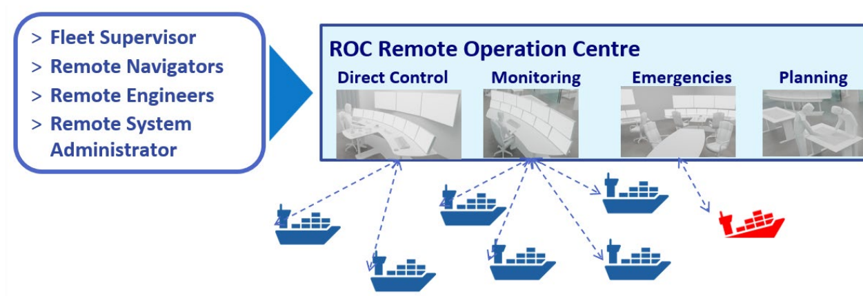
Figure 25: Operational model for MASS without crew on board.
