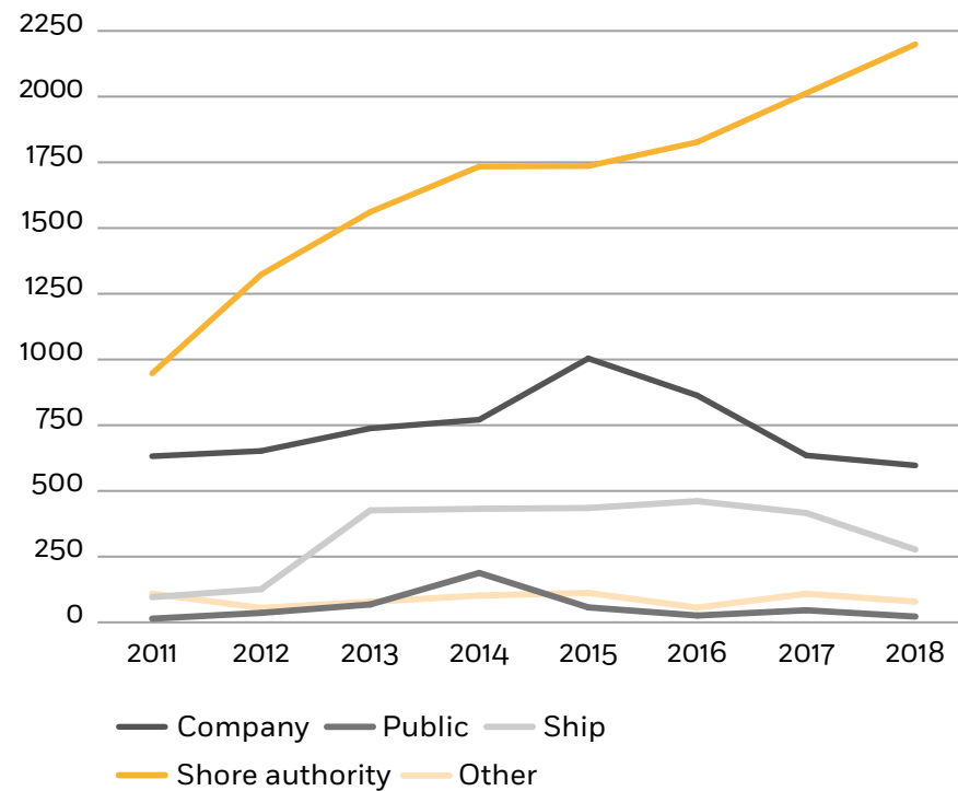
Figure 2.3: Notification entities
