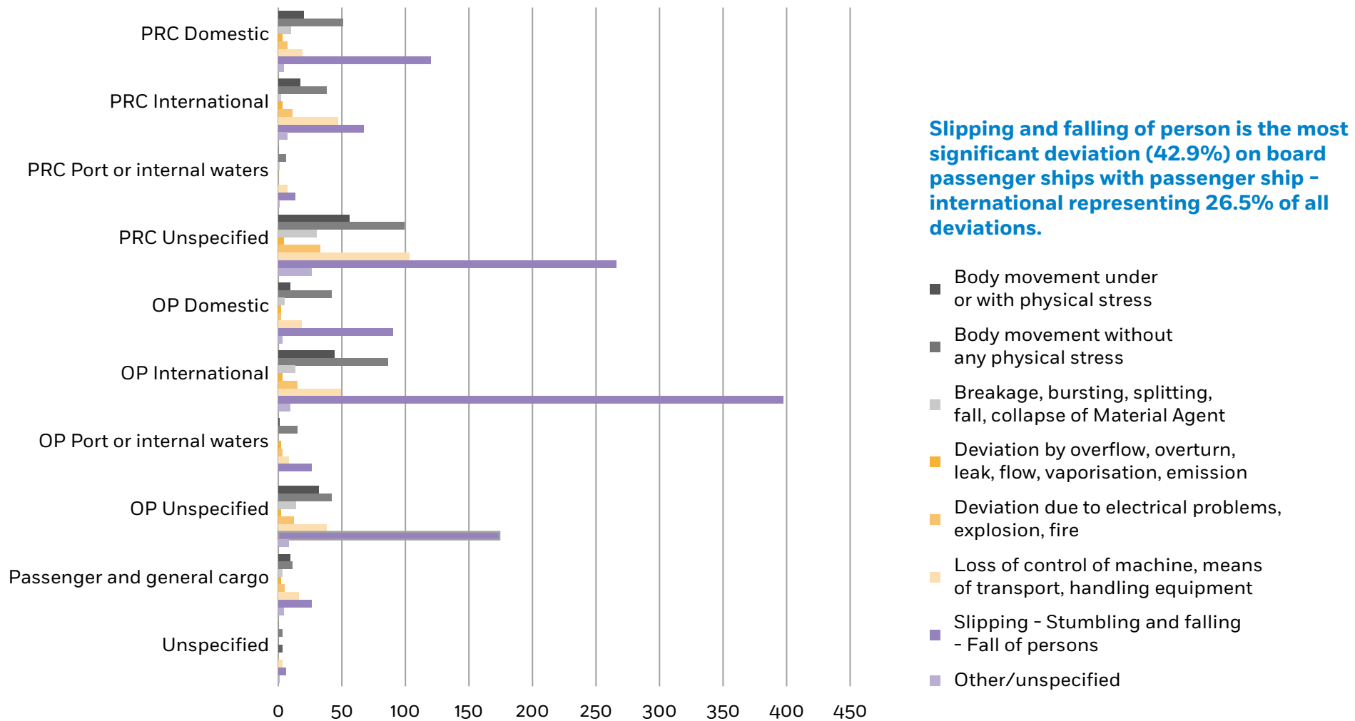
Figure 5.9: Distribution of deviations per passenger ship type for 2011-2018
