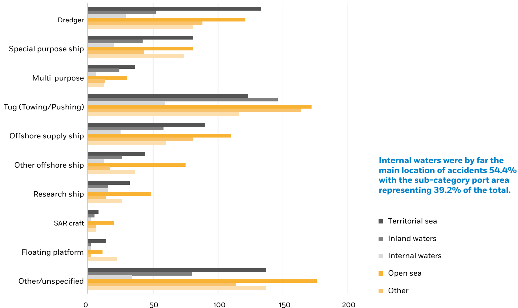
Figure 6.12: Distribution by location of the marine casualties and incidents per service ship type for 2011-2018
